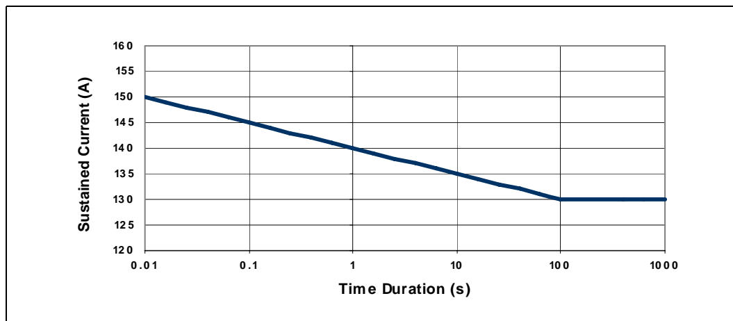
Figure 2-2. Quad-Core Intel® Xeon® Processor X5482 Load Current versus Time
